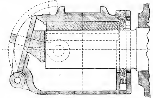
Fig. 5166. Section. THE RAUL JOURNAL-BOX.
